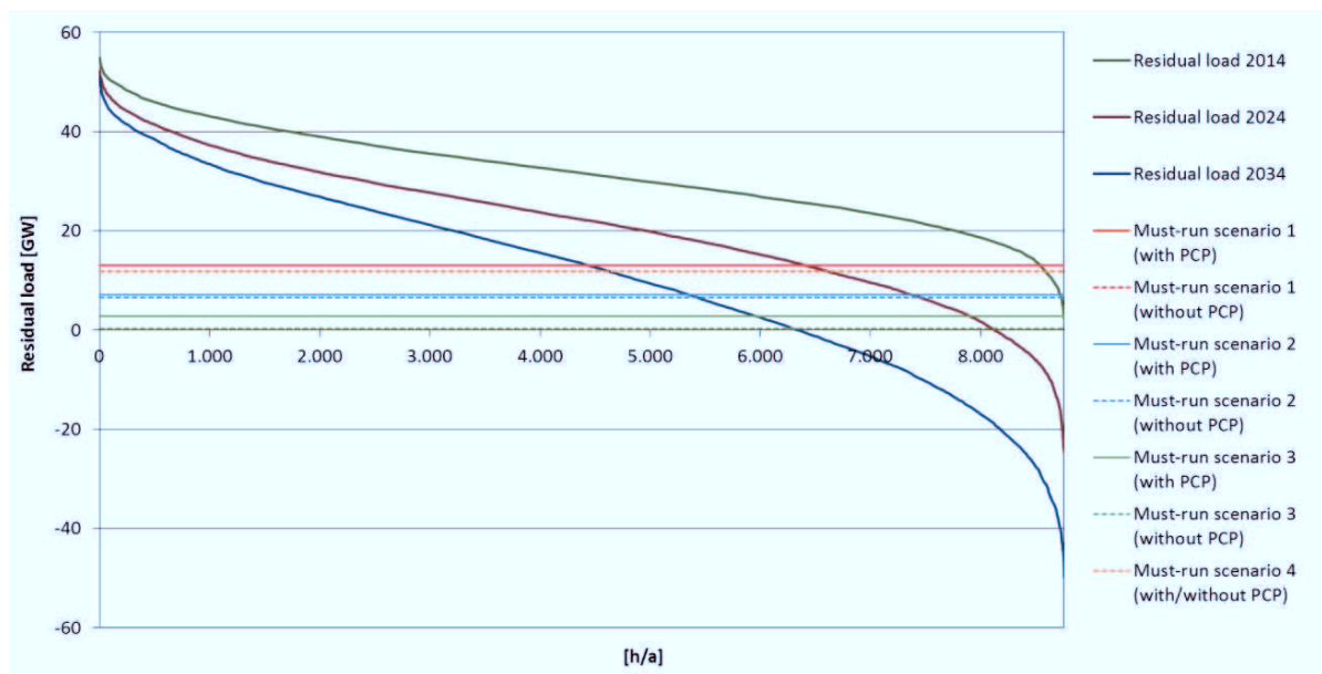
Fig. 2. Residual load and must-run scenarios of a German model CPPs stock providing ancillary services.
