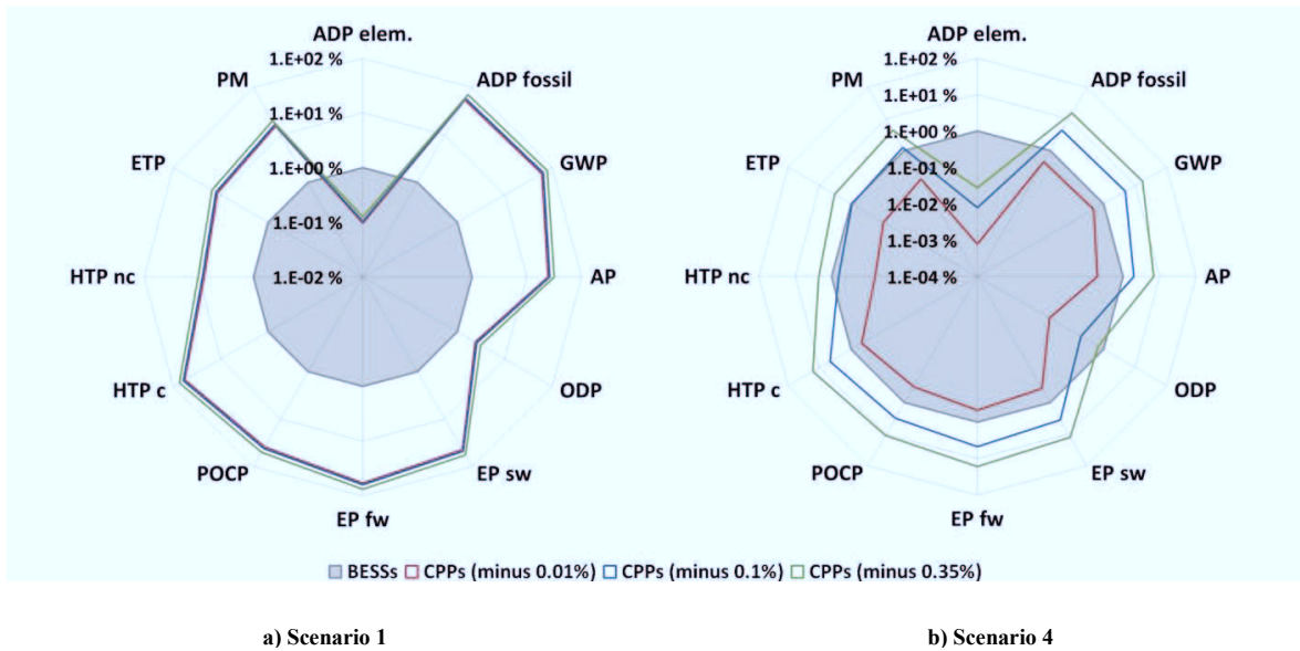
Fig. 4. Comparison of environmental impacts caused by BESSs and CPPs (relative, BESSs = 100 %).
